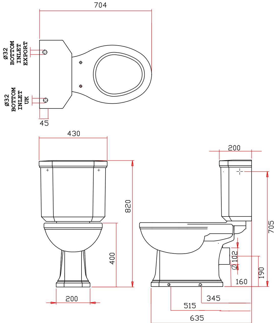
BALASANI CLOSE COUPLED CLOSET AND CISTERN
