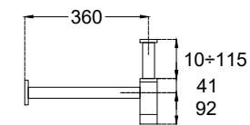
art. 673 sifone compatto | compact siphon
